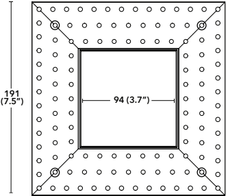
DMS50 Downlight Trimless Adapter Square
