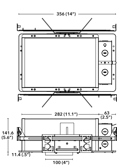
DFR50-IC IC Rated Downlight Frame-In Kit
