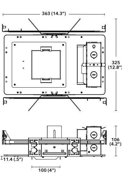
DFR50-T Non IC Thermally Protected Downlight Frame-In Kit
